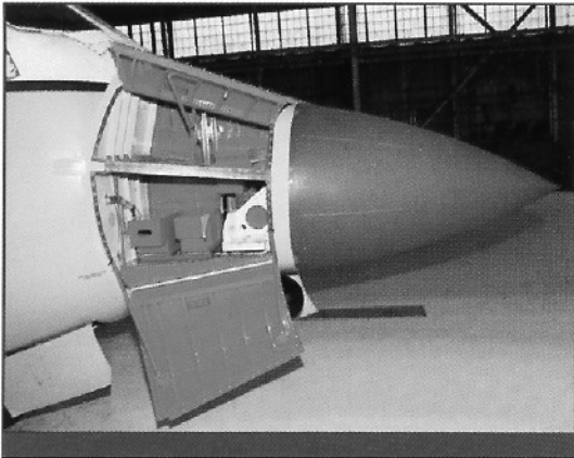
Facilities for Nose-Radar Mounting
